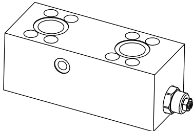
PORTS DIMENSION
